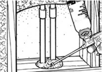
Pipe penetration
